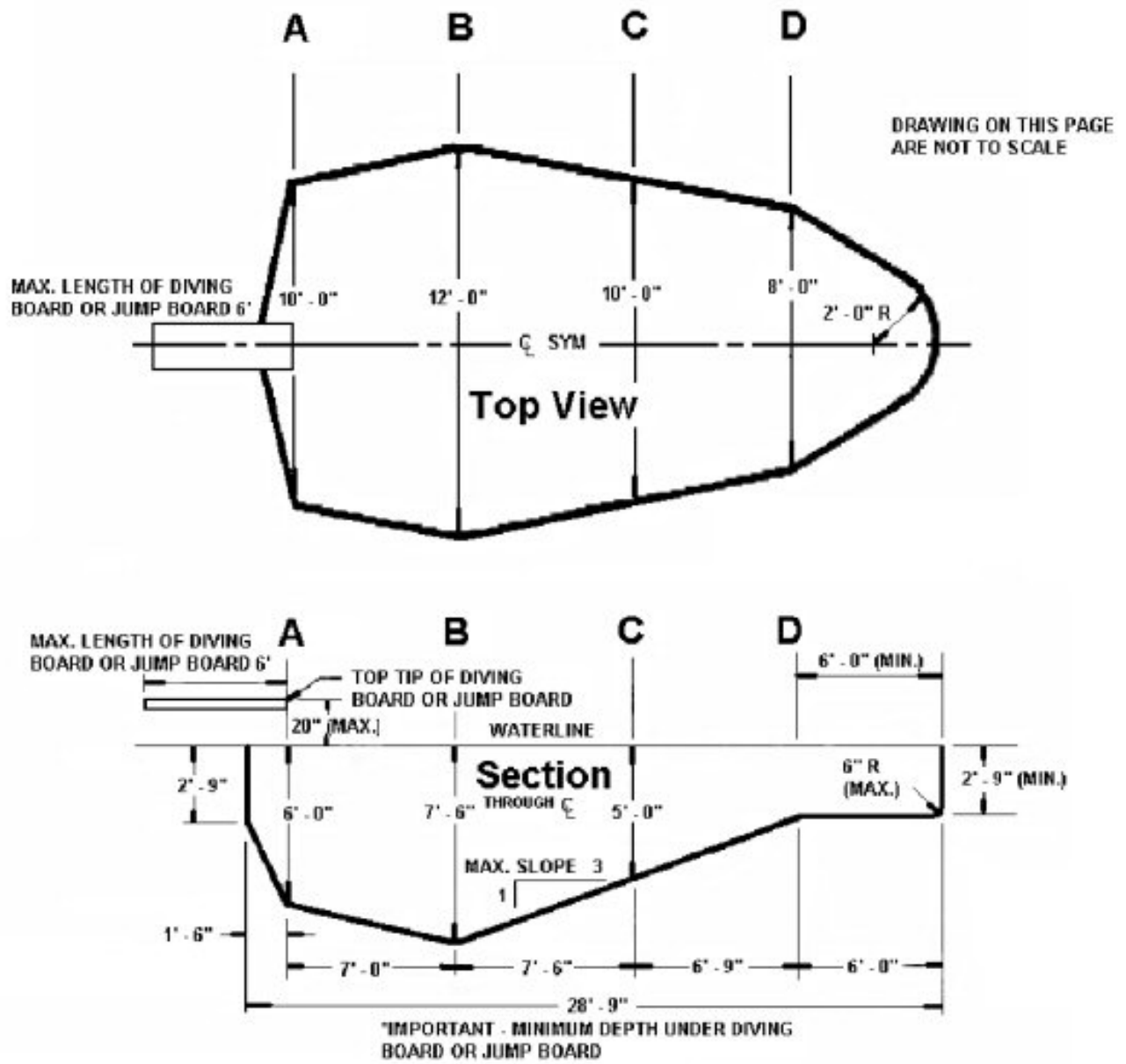
Figure 4-5 Minimal Dimensions - Type 1 Pool
