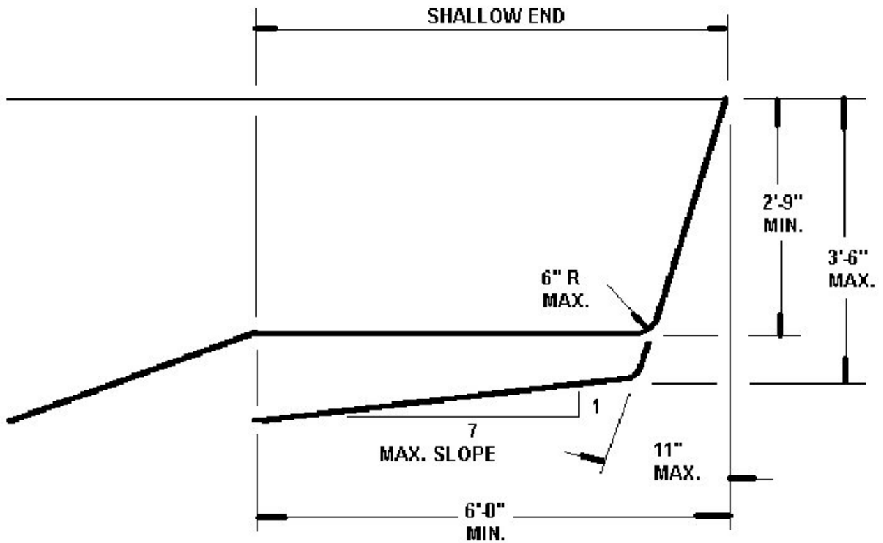
Figure 4-10 Shallow End Detail
