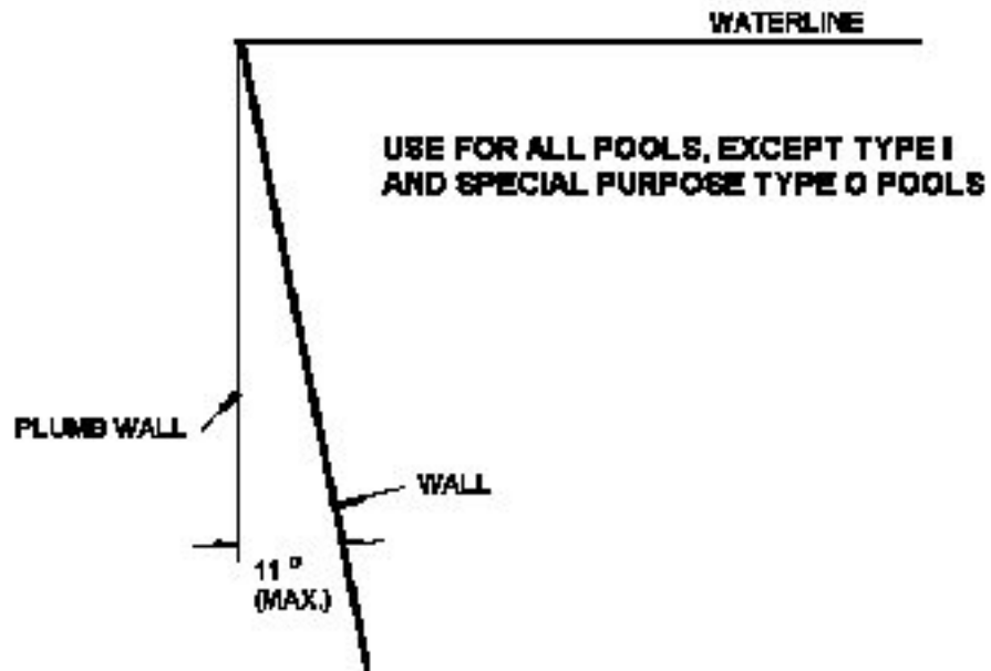
Figure 4-2 Maximum Allowable Wall Slope
